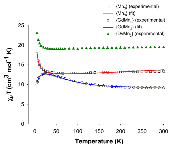
Figure 3. \chi_M T versus T plots for 1-3 in a 1 kG field. The solid lines are the fits of the data; see the text for the fit parameters.
