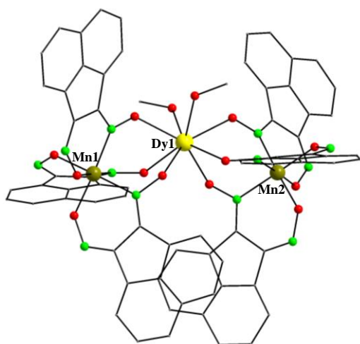
Figure 2. Structure of the anion of 3 . Color scheme: Dy III yellow, Mn IV olive green, N green, O red, C gray.
