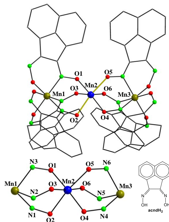
Figure 1. Partially-labeled representations of the anion of 1 (top) and its [Mn 3 (μ-NO) 6 ] 5+ core (bottom). The structure of the ligand acndH 2 is also shown. The Jahn-Teller axial elongations of the central Mn III ion are highlighted with yellow thick bonds. H atoms have been omitted for clarity. Color scheme: Mn III blue, Mn IV olive green, N green, O red, C gray.
